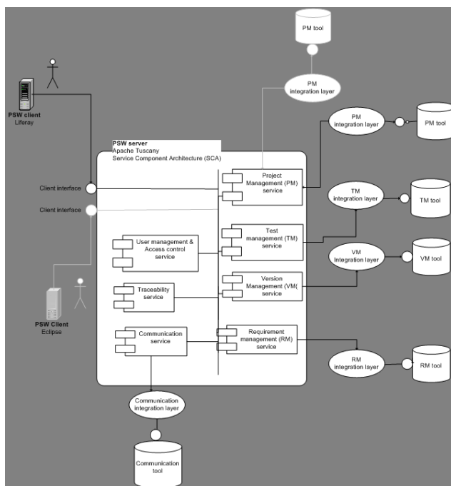
Fig. 2 The architecture of the PSW.
