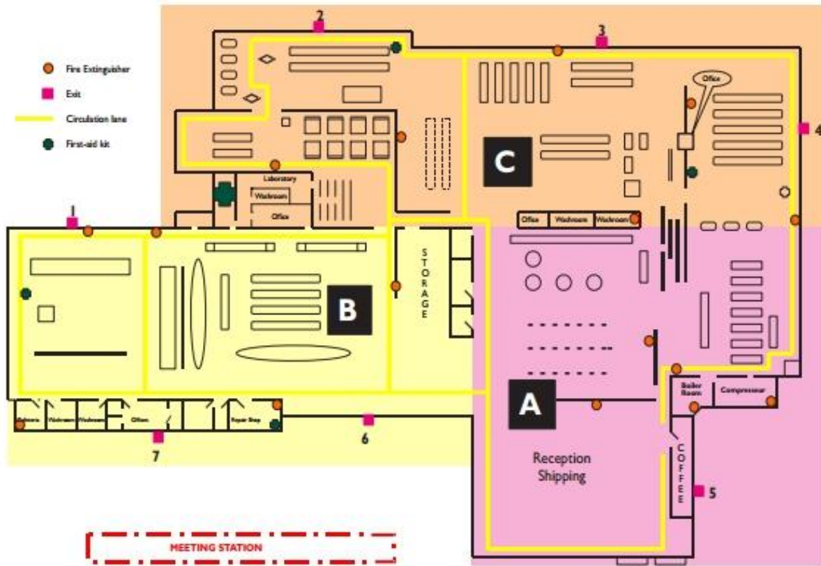
Fig. 2 Evacuation plan of the building based on Prévalex's case study.
