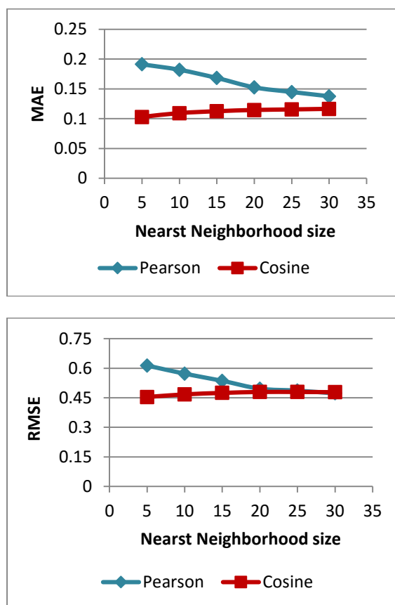
Fig. 4: Impact of neighborhood size on MAE and RMSE
