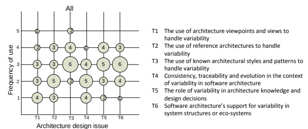
Fig 3. Frequency of use of architecture design issues (frequency of use 1= we don't use, 5 = we use frequently)
