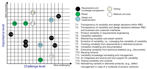
Fig 1. The challenge level and importance of technical variability management topics
