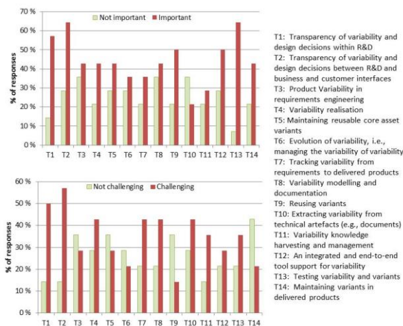
Fig 2. The ratings of importance and challenge level of technical variability management topics
